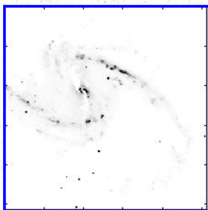
Figure 1. Comparison between the far-UV morphology "predicted" on the basis of optical colors of NGC1365 and the observed morphology from the Ultraviolet Imaging Telescope (UIT). Optical images were obtained from the 2.5m du Pont telescope on Las Campanas, and no noise has been added in order to match the signal-to-noise characteristics of the UIT.
