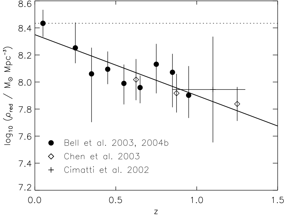
FIGURE 6. The evolution of the stellar mass density in red-sequence galaxies. Stellar masses assume a Kroupa (2001) IMF and H_0 = 70 \text{ km s}^{-1} \text{ Mpc}^{-1} . The local data point is taken from Bell (2003), and data for 0.2 < z < 1.3 is taken from Bell et al. (2004b), Chen et al. (2003), and Cimatti et al. (2002). The solid line shows a rough fit to the total stellar mass density in red-sequence galaxies in the Cole et al. (2000) semi-analytic galaxy formation model. The dotted line shows the expected result if red-sequence galaxies were formed at z \gg 1.5 and simply aged to the present day.
