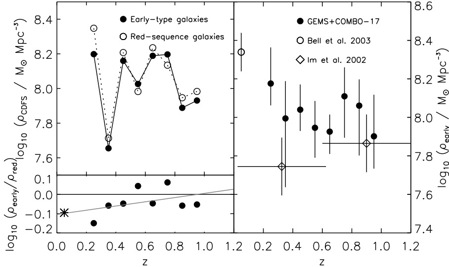
FIGURE 7. The evolution of the stellar mass density in early-type galaxies. Stellar masses assume a Kroupa (2001) IMF and H_0 = 70 \text{ km s}^{-1} \text{ Mpc}^{-1} . The left-hand panel shows the stellar mass densities from GEMS only; solid circles denote early-type galaxies and open circles red-sequence galaxies. The ratio of stellar mass in early-type galaxies to the red sequence is shown in the lower left panel; the asterisk is the local value taken from Bell (2003), and the grey line shows a linear fit to the GEMS data only (RMS \sim 15\% ). The right-hand panel shows the resulting corrected early-type galaxy stellar mass density evolution, where again the local data are taken from Bell (2003), the solid circles denote the GEMS+COMBO-17 result, and the diamonds show results from Im et al.(2002).
