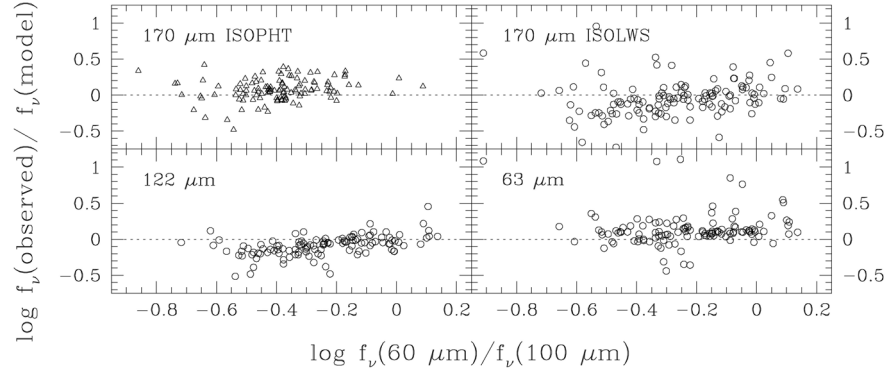
FIGURE 8. Comparison of observed FIR continuum levels observed by ISO with the model predictions of Dale & Helou [18]. The circles derive from the ISO LWS templates and the triangles represent 170 \mu\text{m} data from the ISOPHOT Serendipity Survey (Stickel et al. [81]).
