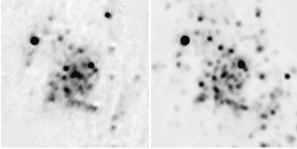
FIGURE 3. Left: Distribution of the localised warm dust component at 60\,\mu\text{m} , F_{60}^1 , in M 33 (Hippelein et al. [42]). This is the scaled difference map 2(F_{60} - 0.165 \times F_{160}) , with the factor 0.165 given by the average flux density ratio F_{60}/F_{170} in the interarm regions. Right: H\alpha map of M 33 convolved to a resolution of 60'' .
