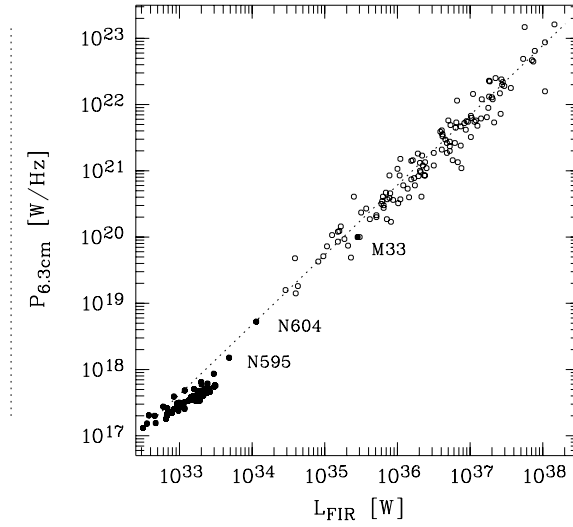
FIGURE 7. Plot of the monochromatic radio luminosity versus the FIR luminosities for M 33 (Hippelein et al. [42]) and its star-forming regions (filled circles) together with the data for the Effelsberg 100-m galaxy sample (Wunderlich et al. [99], open circle). The dotted line has a slope of 1.10 (Wunderlich & Klein [98]).
