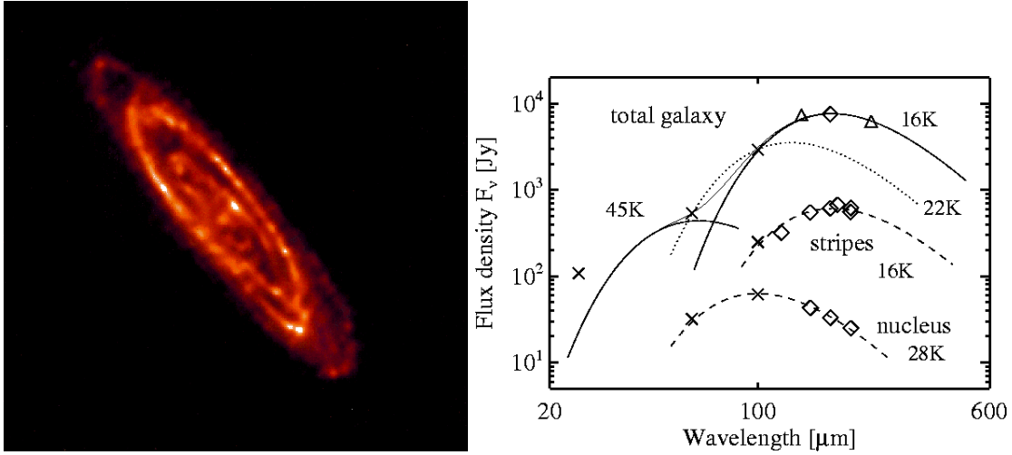
FIGURE 1. Left: ISOPHOT 170\mu\text{m} map of M 31 (Haas et al. [34]), with an angular resolution of 1.3'' . North is towards the top, and East is towards the left. The field size is 2.9 \times 2.9 degrees. Right: Infrared SED of M 31 (Haas et al. [34]). The data are shown by symbols (diamonds ISO, crosses IRAS, triangles DIRBE) with the size being larger than the errors. The blackbody curves with emissivity proportional to \lambda^{-2} are shown by lines. The dotted line with T=22\text{ K} through the IRAS 60 and 100\mu\text{m} data points indicates what one would extrapolate from this wavelength range alone without any further assumptions.
