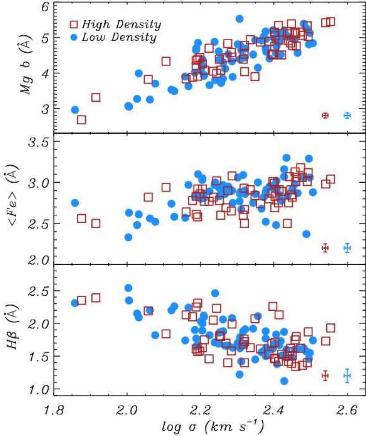
Fig. 15.— Dependence of E/S0 spectral indices on \sigma and environment from Thomas et al. (2005). Filled blue circles are low density points; open red squares are high density points. Top panel is the Mg b indicator ( \alpha abundance), middle panel is the \langle Fe \rangle indicator (iron abundance), and bottom panel is H \beta (an age indicator). Typical uncertainties in the measurements are shown in the lower right corners.
