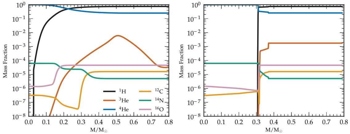
Figure 12. Abundance profiles in a 0.8M_\odot model with Z = 0.00015 (see also Figure 9). The left panel shows a time just after core hydrogen exhaustion and the right panel shows the situation soon after the maximum inward penetration of the convective envelope. At this time the hydrogen burning shell is at m(r) \approx 0.31M_\odot and the convective envelope has homogenized all abundances beyond m(r) \approx 0.36M_\odot . The initial ^3\text{He} profile has been homogenised throughout the mixed region, resulting in an increase in the surface value, which is then returned to the interstellar medium through winds, unless some extra-mixing process can destroy it first.
