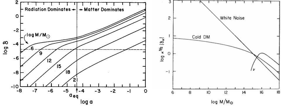
Figure 1.1 The origin of the CDM spectrum of density fluctuations. Left panel: Fluctuations corresponding to mass scales 10^6 M_\odot , 10^9 M_\odot , etc., grow proportionally to the square of scale factor a when they are outside the horizon, and when they enter the horizon (cross the horizontal dashed line) the growth of the fluctuation amplitude \delta is much slower if they enter when the Universe is radiation dominated (i.e., a < a_{\text{eq}} ). Fluctuations on mass scales > 10^{15} M_\odot enter the horizon after it becomes matter dominated, so their growth is proportional to scale factor a ; that explains the larger separation between amplitudes for such higher-mass fluctuations. (From a 1983 conference presentation Primack and Blumenthal (1984), reprinted in Primack (1984).) Right panel: The resulting CDM fluctuation spectrum ( \kappa^{3/2} |\delta_\kappa| = \Delta M/M ) is contrasted with a \delta \propto \kappa^0 white noise (Poisson) spectrum with the same power at all wavelengths (where wave number \kappa is as usual related to wavelength \lambda by \kappa = 2\pi/\lambda ), and with the hot dark matter spectrum if the dark matter were light neutrinos ( \nu ) which is cut off on galaxy mass scales by free-streaming. (From Blumenthal et al. (1984). This calculation assumed that the primordial fluctuations are scale-invariant (Zel'dovich) and that \Omega_{\text{matter}} = 1 and Hubble parameter h = 1 .)
