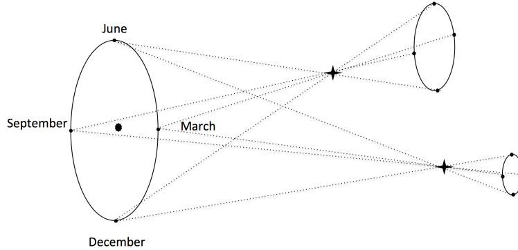
Figure 2: The parallactic motion for a nearby and a distant star.
