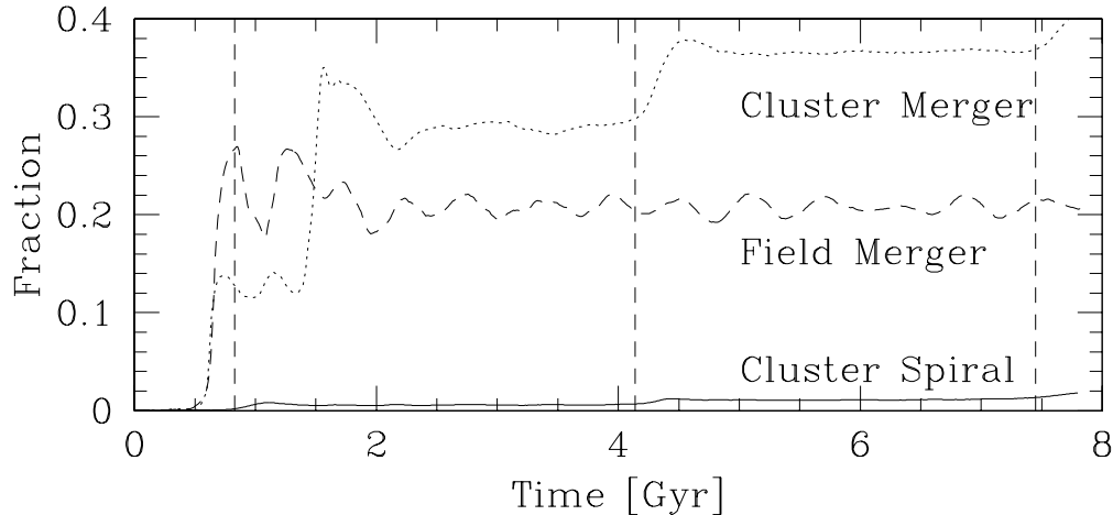
Figure 4. Material stripped to large radius ( r > 35 kpc) for the isolated merger, the cluster merger, and an isolated spiral orbiting in the cluster potential. Cluster peri passages are shown as dashed lines. Note that most of the tidal material in the isolated merger remains bound to the remnant, while it is unbound in the cluster merger.
