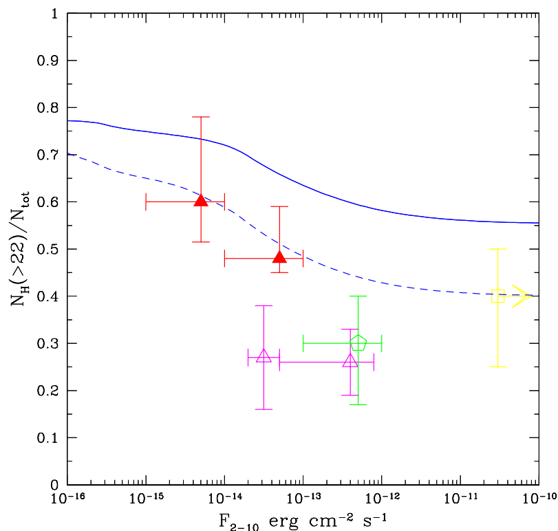
Figure 8.4. Expected fraction of sources with absorption column densities larger than 10^{22} \text{ cm}^{-2} vs. 2–10 keV flux for a model without ( solid line ) and with ( dashed line ) Compton thick sources. Points and associated error bars correspond to the observed fraction of absorbed sources in different X-ray surveys: open square at bright X-ray fluxes is from the HEAO1-A2 AGN sample of Piccinotti et al. (1982), open hexagon is from the ASCA Large Sky Survey (Akiyama et al. 2000), open triangles are from XMM-Newton observations (Piconcelli et al. 2002), and filled triangles are from Chandra observations (Brusa 2004).
