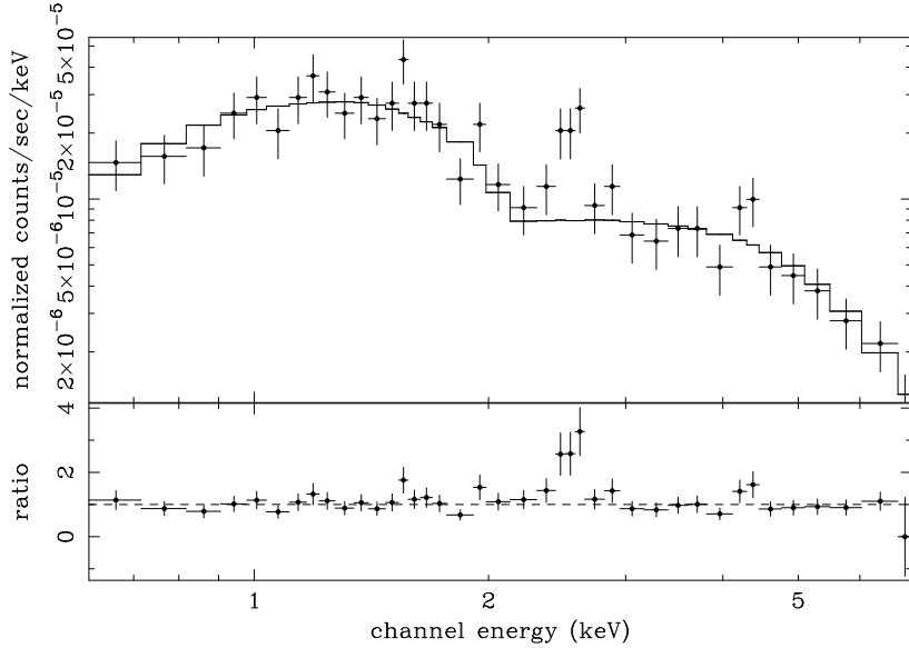
Figure 8.8. Simulated spectrum of a reflection dominated F_{2-10 \text{ keV}} \sim 10^{-15} \text{ ergs cm}^{-2} \text{ s}^{-1} source at z = 1.5 , as would be seen with an ultradeep 10 Ms Chandra observation. Input parameters are a flat power law with \Gamma=1 plus an iron line with an observed EW of 600 eV. The line feature is clearly seen in the residuals (bottom panel) of a single power law fit.
