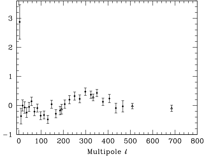
Figure 3: Cross power spectrum of the temperature anisotropies and E-mode polarization signal from WMAP (points), together with some estimates from DASI (triangles) which extend to higher \ell . Note that the DASI bands are much wider in \ell than those of WMAP . Also note that the y -axis is not multiplied by the additional \ell , which helps to show both the large and small angular scale features.
