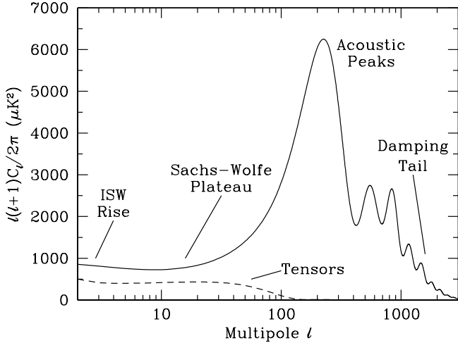
Figure 1: Plot of the theoretical CMB anisotropy power spectrum, using a standard \Lambda CDM model from CMBFAST . The x -axis is logarithmic here. The regions are labeled as in the text: the ISW Rise; Sachs-Wolfe Plateau; Acoustic Peaks; and Damping Tail. Also shown is the shape of the tensor (gravity wave) contribution, with an arbitrary normalization.
