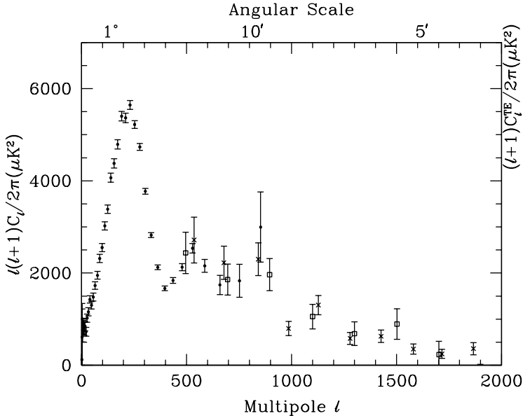
Figure 2: Band-power estimates from the WMAP , CBI, and ACBAR experiments. The WMAP data are the points, while squares are CBI and crosses ACBAR. We have shown only CBI and ACBAR data relevant for \ell > 500 , and both experiments also probe to higher \ell than shown. This plot represents only a fraction of experimental results, with several other data-sets being of similar quality. The multipole axis here is linear, so the Sachs-Wolfe plateau is hard to see. The acoustic peaks and damping region are very clearly observed, with no need for a theoretical curve to guide the eye.
