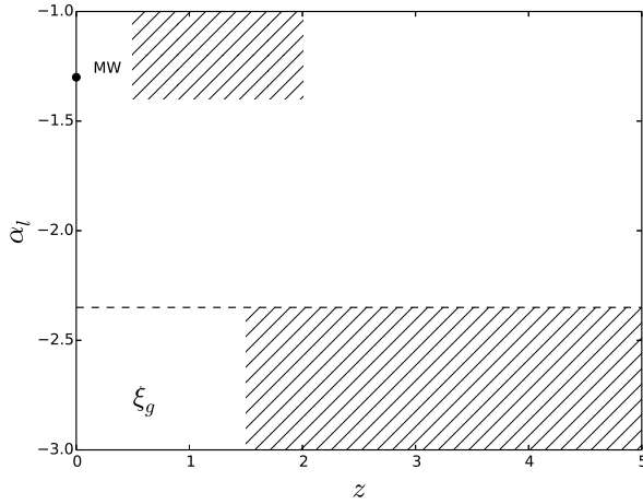
Figure 10. The low mass slope of the IMF ( \alpha_l ) as a function of redshift, representative of the formation time of the stars involved. The Kroupa (2001) value for the Milky Way is shown as the data point, and the range of values for \alpha_l from Bastian et al. (2010) for Milky Way stars is shown as the upper hatched region, corresponding broadly to formation (look-back) times spanning 5 \lesssim t/\text{Gyr} \lesssim 10 . The lower hatched region shows the steep low mass IMF slopes, at formation times approximately 9.5 \lesssim t/\text{Gyr} \lesssim 12.3 , for the passive galaxies discussed in § 5.3 above. Note that the broad range of \alpha_l for these galaxies is indicated, and potential dependencies on \sigma or [M/H] are not represented.
