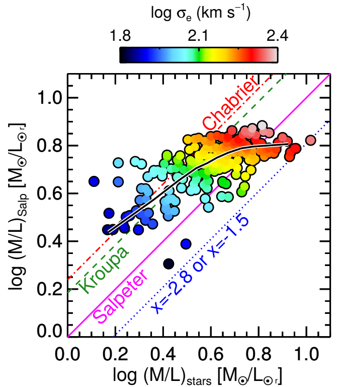
Figure 6. The mass-to-light ratio for the stellar component of ATLAS3D galaxies estimated using dynamical models, (M/L)_{\text{stars}} , compared to that estimated from spectral fitting using SPS models assuming a fixed Salpeter IMF, (M/L)_{\text{Salp}} . This demonstrates the trend for the high mass-to-light, or high velocity dispersion, galaxies in this sample to favour IMFs with an excess of mass compared to the IMFs of Chabrier (2003a) or Kroupa (2001) , approaching and exceeding that from a Salpeter slope over the full mass range (an excess of low mass stars). See Cappellari et al. (2013) for details. Reproduced from Figure 11 of “The ATLAS3D project – XX. Mass-size and mass- \sigma distributions of early-type galaxies: bulge fraction drives kinematics, mass-to-light ratio, molecular gas fraction and stellar initial mass function,” Cappellari et al. (2013) .
