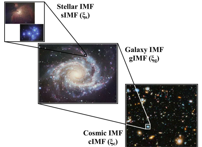
Figure 7. A framework to aid in clarifying discussions of the IMF. If the IMF is not universal, then the sIMF, gIMF and cIMF are not necessarily the same, and all may have a time-dependence. Different measurement techniques and observational samples probe these different quantities, and what has been referred to uniformly in published work to date as “the IMF” conflates these distinct properties. This may well contribute to much of the current tension between different IMF estimates in different contexts.
