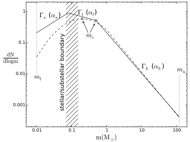
Figure 1. An illustration of the key aspects of the IMF as it has been parameterised, either as a piecewise series of power-law segments (e.g., Kroupa 2001) or a log-normal at low masses with a power-law tail at high masses (e.g., Chabrier 2003a).
