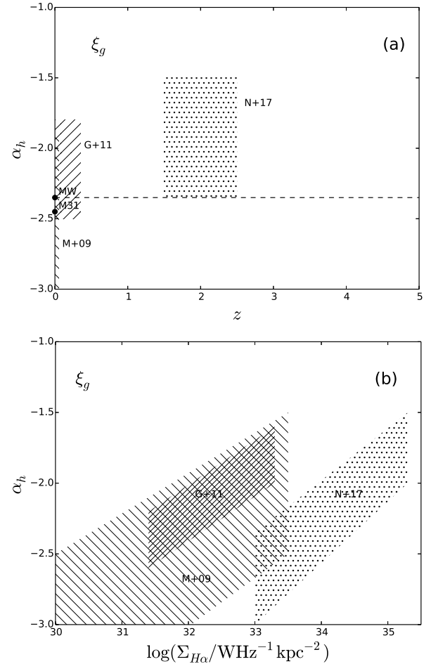
Figure 9. (a) The possible variation in \alpha_h for \xi_g from Meurer et al. (2009), Gunawardhana et al. (2011), and Nanayakkara et al. (2017), shown as hatched and dotted regions. The dashed line is the Salpeter slope ( \alpha_h = -2.35 ). Values for the Milky Way (MW) and M31 (Weisz et al. 2015) are also shown. Note that the full range of \alpha_h is indicated, and the dependencies on sSFR or other physical property are not represented here. (b) The approximate dependence of \alpha_h on H \alpha surface density, inferred from each of Gunawardhana et al. (2011), Meurer et al. (2009) and Nanayakkara et al. (2017).
