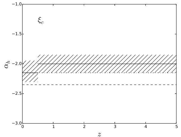
Figure 8. The possible variation in \alpha_h for \xi_c from Wilkins et al. (2008b) (solid lines and hatched regions). The dashed line is the Salpeter slope ( \alpha_h = -2.35 ), and represents the “universal” IMF from Madau & Dickinson (2014) . The dot-dashed line is \alpha_h = -2.15 from Baldry & Glazebrook (2003) .
