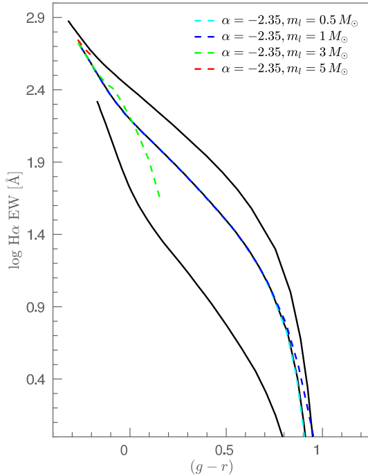
Figure 4. The IMF diagnostic used by Gunawardhana et al. (2011) to identify variations in the slope of the high mass ( m > 0.5 M_{\odot} ) IMF. The black solid lines show the evolutionary tracks expected for galaxies with, from top to bottom, \alpha_h = -2, -2.35, -3 . The additional tracks (dashed coloured lines) illustrate the effect of a fixed high mass slope ( \alpha = -2.35 ) but varying m_l . The tracks become shorter as m_l increases, due to the shorter lifetimes of the higher mass stars. Figure courtesy of M. Gunawardhana.
