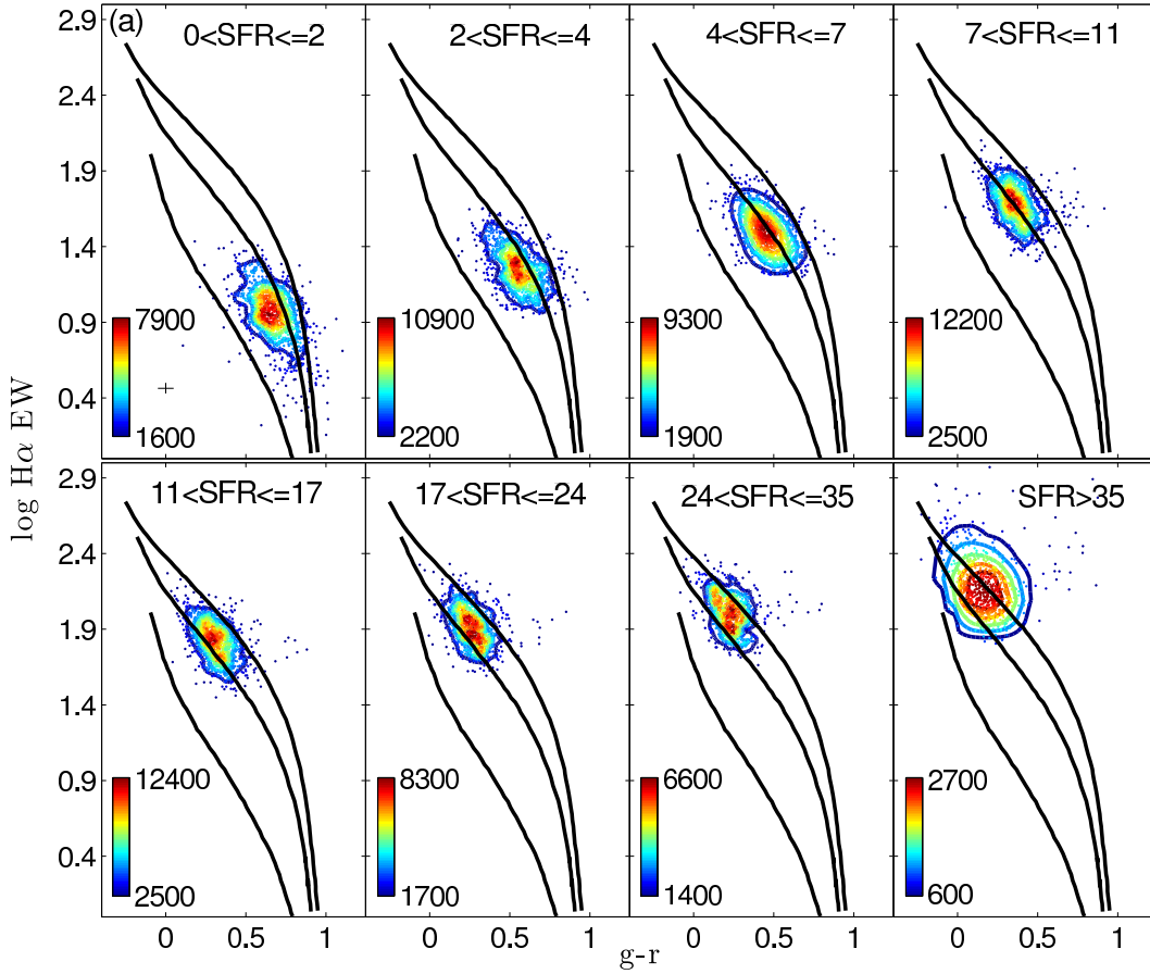
Figure 3. Following Kennicutt (1983) and Hoversten & Glazebrook (2008) , this diagnostic shows how IMFs with different \alpha_h can be discriminated using the equivalent width of H \alpha and an optical colour, in this case (g-r) . The solid tracks are the evolutionary paths followed through a star formation event, showing (top to bottom) the location expected for \alpha_h = -2 , \alpha_h = -2.35 , \alpha_h = -3 . The data correspond to galaxies in the highest redshift bin of the three volume limited samples, with \langle z \rangle = 0.29 , split into eight bins of SFR. This illustrates the tendency for the higher SFR systems to favour IMFs with flatter high mass slopes (more positive \alpha_h ). See Gunawardhana et al. (2011) for details. Reproduced from Figure 6a of “Galaxy and Mass Assembly (GAMA): the star formation rate dependence of the stellar initial mass function,” Gunawardhana et al. (2011) .
