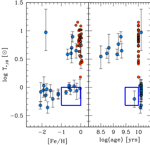
Figure 2. The stellar mass-to-light ratio at 10 Gyr, \Upsilon_{*,10} , as a function of metallicity and age, showing two distinct populations. Clusters (blue data points) with younger ages, or higher metallicities, tend to show higher mass-to-light ratios, indicative of an IMF similar to Salpeter ( \alpha = -2.35 ) over the full mass range. Older, more metal-poor, clusters have mass-to-light ratios consistent with an IMF having proportionally fewer low mass stars, such as that of Kroupa et al. (1993). The red data points represent the mass-to-light ratios for early type galaxies, while the blue box indicates the range of \Upsilon_{*,10} for disk galaxies. See Zaritsky et al. (2014b) for details. (Figure 9 of “Evidence for two distinct stellar initial mass functions: Probing for clues to the dichotomy,” Zaritsky et al. (2014b), © AAS. Reproduced with permission.)
