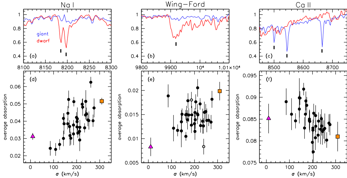
Figure 5. Three spectral regions showing features sensitive to the presence or absence of low mass stars (upper panels), and the trend in the absorption strength of those features seen with velocity dispersion of the galaxies (lower panels). This demonstrates that galaxies with higher velocity dispersion, and hence higher stellar mass, have a tendency to favour an excess of dwarf, or low mass, stars. See van Dokkum & Conroy (2012) for details. (Figure 10 of “The stellar initial mass function in early-type galaxies from absorption line spectroscopy. I. Data and empirical trends,” van Dokkum & Conroy (2012) , © AAS. Reproduced with permission.)
