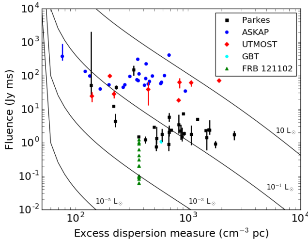
Fig. 16 Fluence–dispersion measure distribution for the currently observed sample overlaid with lines of isotropic equivalent luminosity values assuming a contribution of DM_{\text{Host}} = 50 \text{ cm}^{-3} \text{ pc} . The recent detections from CHIME/FRB have been omitted (see text).
