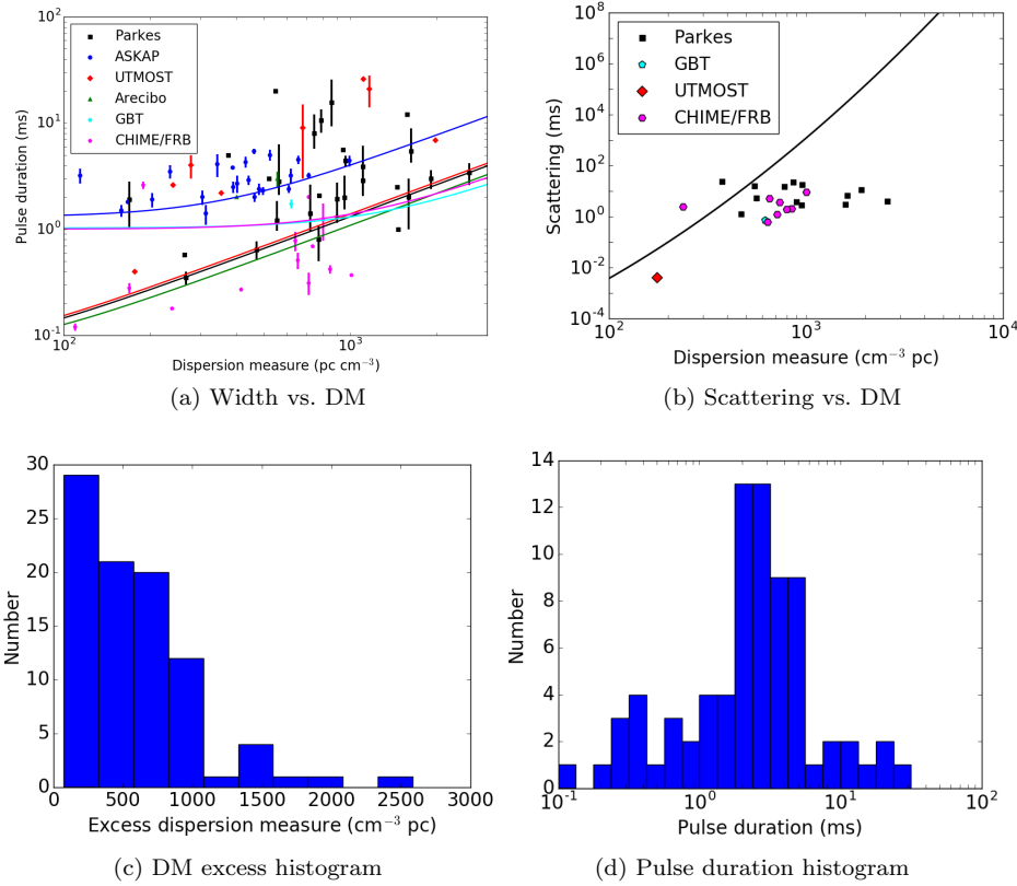
Fig. 13 The properties of the catalogued FRB population. (a) The pulse duration (width) versus DM. Solid lines represent temporal broadening from DM smearing in an individual frequency channel combined with the sampling time for different telescopes. In the case of FRBs from CHIME, plotted widths have been obtained through modeling and are not the observed FRB widths from the instrument. (b) Scattering timescale versus DM for all FRBs where scattering has been measured. The curve shows the DM-scattering relation for pulsars in the Galaxy derived by Bhat et al. (2004). FRBs are under-scattered relative to Galactic pulsars of similar DMs. (c) A histogram of the DM excess compared to the expected Galactic maximum along the line of sight. (d) A histogram of the pulse durations. For panels (a) and (b) colors correspond to the Parkes (black), ASKAP (blue), Arecibo (green), UTMOST (red), GBT (cyan) and CHIME (pink) telescopes.
