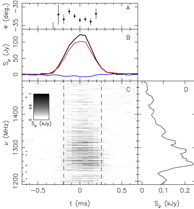
Fig. 4 Apparent scintillation seen in FRB 150807. Panel C shows a dedispersed dynamic spectrum of the burst at 390-kHz spectral resolution. The inferred scintillation bandwidth is 100 \pm 50 kHz. Panel B shows the frequency-averaged burst profile with total intensity (black), linearly polarized signal (red), and circularly polarized signal (blue). Panel A shows the polarization angle across the burst, and Panel D shows a smoothed version of the burst spectrum. Fig. 1 from Ravi et al. (2016).
