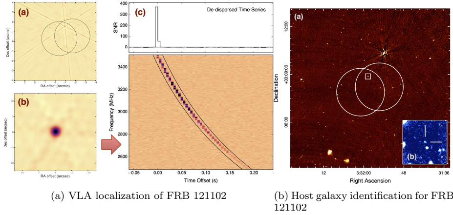
Fig. 10 Left: Using the VLA, repeating bursts from FRB 121102 were localized to sub-arcsecond precision using interferometric techniques. Right: The localization allowed for the identification of the host galaxy at radio and optical (inset) wavelengths. Figures 1 and 2 from Chatterjee et al. (2017).
