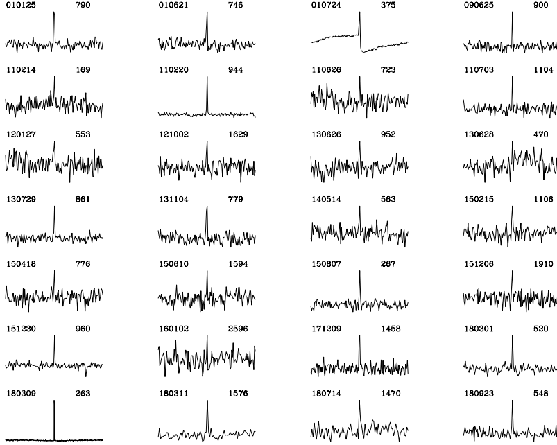
Fig. 3 Compilation showing the first twenty-eight FRBs discovered using the Parkes telescope. The detections are arranged in order of date. Each light curve shows a 2-s window around the pulse. Following gamma-ray burst notation, the FRBs are named in YYMMDD format to indicate the year (YY) month (MM) and day (DD) on which the burst was detected. Also listed to the right of each pulse are the observed dispersion measures (DMs) in units of \text{cm}^{-3} \text{ pc} .
