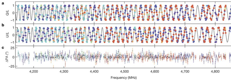
Fig. 6 Faraday rotation seen in FRB 121102. Panels a and b show the values of the Stokes Q and U parameters across the measured frequency range, normalized to the total linear intensity. Panel c shows the residuals compared to a best-fit Faraday rotation model. The various colors represent measurements from separate bursts detected in the same observing session. Fig. 2 from Michilli et al. (2018a).
