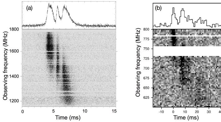
Fig. 11 De-dispersed spectra of individual bursts from (a) the repeating FRB 121102 at 1.4 GHz using Arecibo, and (b) the repeating FRB 180814.J0422+73 discovered with CHIME at 700 MHz. Both repeating sources have some bursts that show distinct sub-burst structure with descending center frequencies over time. Horizontal bands in both spectra are due to narrow-band RFI excision in the data. FRB 121102 data from Hessels et al. (2018). FRB 180814.J0422+73 data from CHIME/FRB Collaboration et al. (2019a).
