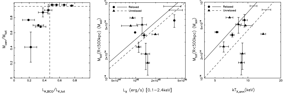
Fig. 27. Left Panel: Central mass fraction (a measure of the dominance of the central dark matter halo), M_{cen}/M_{tot} versus central K-band luminosity fraction (measures the dominance of the central galaxy), L_{K,BCG}/L_{K,tot} . There is a remarkably clean separation between a homogeneous population of centrally concentrated clusters ( M_{cen}/M_{tot} > 0.95 , L_{K,BCG}/L_{K,tot} > \sim 0.55 ) and a much more diverse population of less concentrated clusters. Center & Right Panels: Mass- L_X and Mass- T_X relations. The solid and dashed lines show the best-fit relations normalized by the relaxed and unrelaxed clusters respectively. The error bars on each line show the uncertainty on the normalizations. The scatter in the Mass- L_X relation appears to be symmetric; in the mass- T_X relation the normalization of the unrelaxed clusters appears to be 40% hotter than the relaxed clusters at 2\sigma significance. Figures from Smith et al. (2005).
