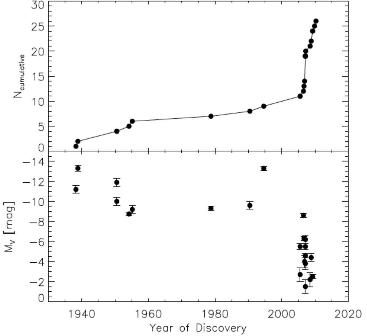
Fig. 1.— Cumulative number (top) and luminosity (bottom) of known dwarf spheroidal satellites of the Milky Way, versus year of publication of discovery paper (Shapley 1938a,b; Harrington & Wilson 1950; Wilson 1955; Cannon et al. 1977; Irwin et al. 1990; Ibata et al. 1994; Willman et al. 2005b,a; Belokurov et al. 2006; Zucker et al. 2006b,a; Belokurov et al. 2007; Irwin et al. 2007; Walsh et al. 2007; Belokurov et al. 2008; Belokurov et al. 2009; Grillmair 2009; Watkins et al. 2009; Belokurov et al. 2010).
