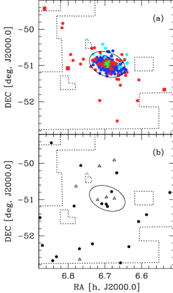
Fig. 6.— Extended stellar structure of the Carina dSph, from narrow-band photometry and spectroscopy of Muñoz et al. (2006, reproduced by permission of the American Astronomical Society). The top/bottom panels show sky positions of red giant candidates confirmed as Carina members/nonmembers. Ellipses mark Carina’s limiting radius, R_K (Equation 1), determined from smooth fits to star count data. The extension of faint stellar structure at R \gtrsim 3R_K suggests tidal interaction (Section 3.2). Muñoz et al. (2005) report similar results for Ursa Minor.
