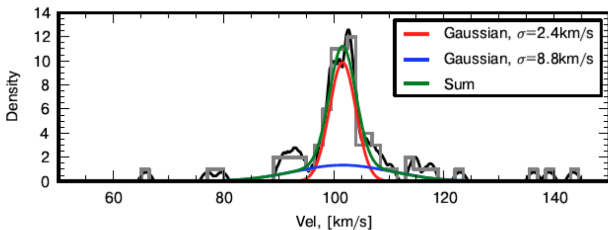
Fig. 16.— Velocity distribution of the Boötes I dSph, from the VLT/FLAMES data of Koposov et al. (2011b, reproduced by permission of the American Astronomical Society), not including 11 stars observed to have significant velocity variability. In the best-fitting two-Gaussian model, 70% of the stars belong to a ‘cold’ component with \sigma \sim 2 \text{ km s}^{-1} and the rest belong to a hotter component with \sigma \sim 9 \text{ km s}^{-1} .
