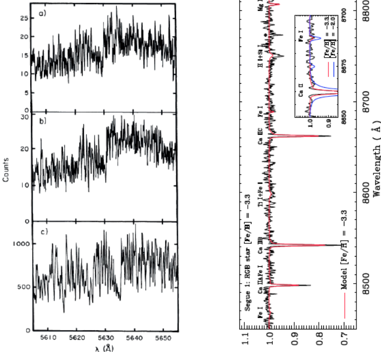
Fig. 8.— Examples of spectra for individual dSph stars. Left : MMT echelle spectra ( R \sim 30000 ) for three carbon stars in Draco, used for the first measurement of a dSph velocity dispersion (Aaronson 1983, reproduced by permission of the American Astronomical Society). Right : Keck/DEIMOS spectrum ( R \sim 6000 ) for the brightest red giant in Segue 1 (Geha et al. 2009, reproduced by permission of the American Astronomical Society), with absorption features labeled and best-fitting model overplotted.
