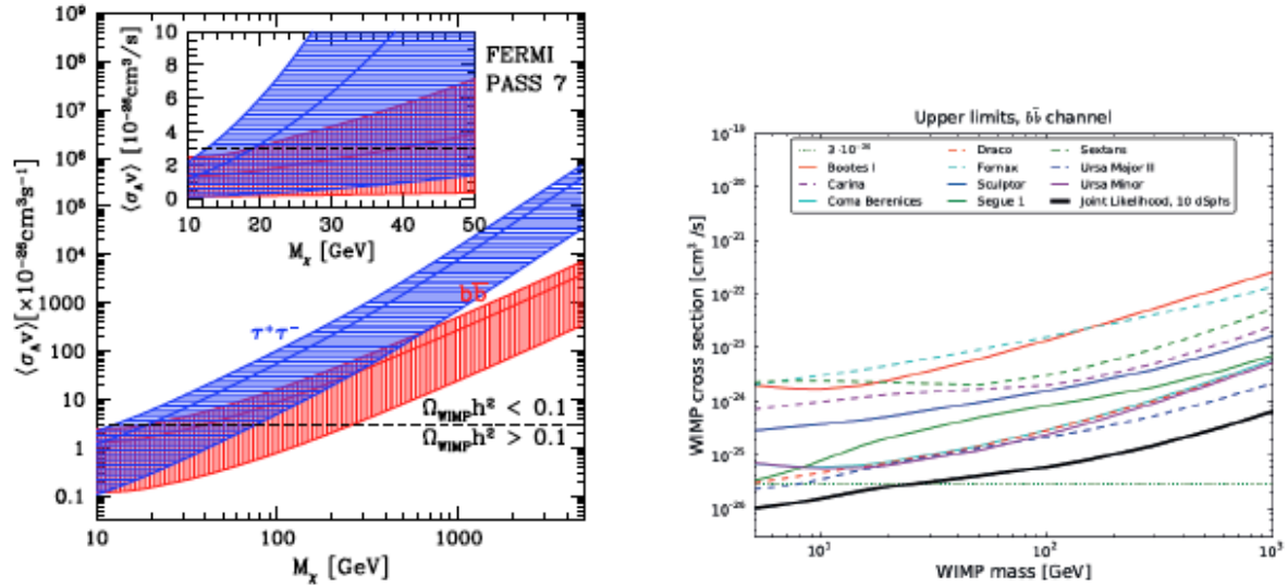
Fig. 22.— Exclusion of WIMP self-annihilation cross sections, based on Fermi-LAT non-detections (2-year data) of gamma-rays in the Milky Way’s dSph satellites (reprinted with permission from Geringer-Sameth & Koushiappas, Phys. Rev. Lett. 107, 241303 (2011; left) and Ackermann et al. (The Fermi Collaboration), Phys. Rev. Lett. 107, 241302 (2011; right), Copyright 2011 by the American Physical Society).
