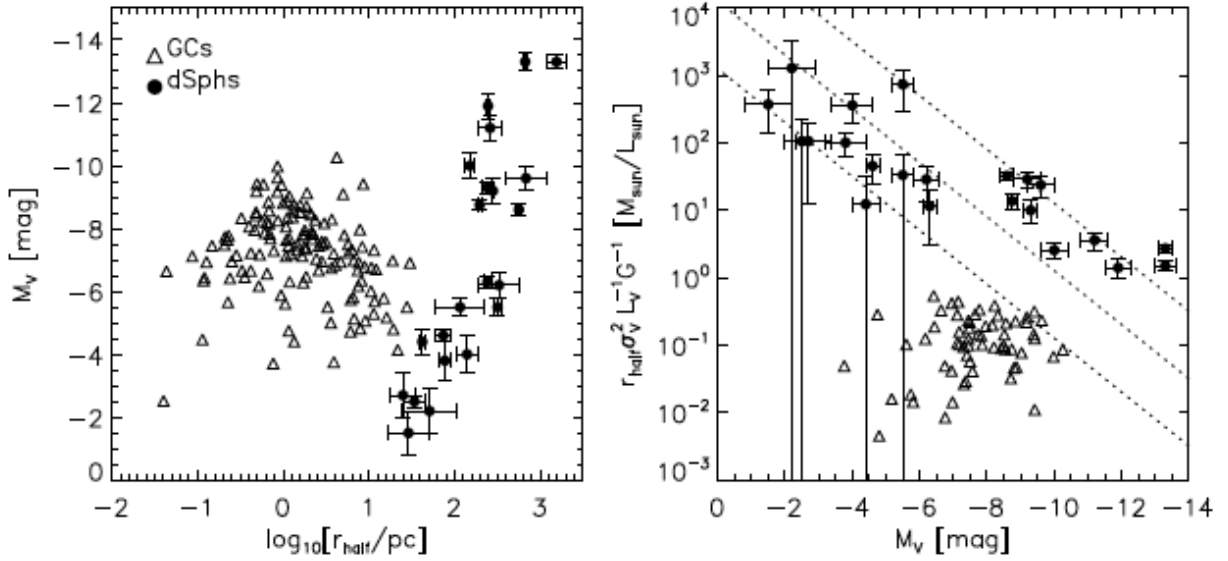
Fig. 13.— Left : Luminosity versus size (updated from Belokurov et al. 2007; Gilmore et al. 2007; Martin et al. 2008), for Milky Way satellites including objects classified as globular clusters (open triangles; data from Harris (1996, 2010 edition)) and dwarf spheroidals (filled circles with error bars; data from compilations by Irwin & Hatzidimitriou 1995; Mateo 1998; Martin et al. 2008; Sand et al. 2011). The apparent lack of objects toward low luminosity and large size is a selection effect that reflects the surface-brightness limit of the SDSS survey (Koposov et al. 2008). Right : Dynamical mass-to-light ratio (modulo a constant scale factor) versus luminosity. Updated from Mateo et al. (1993); Mateo (1998); Simon & Geha (2007); Geha et al. (2009). Dotted lines correspond to constant masses of 10^5 M_{\odot} , 10^6 M_{\odot} and 10^7 M_{\odot} .
