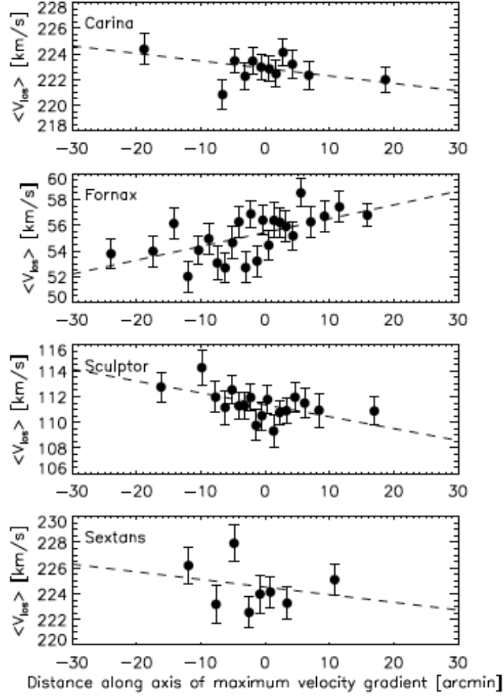
Fig. 14.— Line-of-sight velocity gradients in the Milky Way’s ‘classical’ dSph satellites. Panels display mean velocity as a function of distance along the axis corresponding to the maximum velocity gradient, from the samples of Walker, Mateo & Olszewski (2009). The observed gradients give rise to maximum amplitudes R_{\max} dV/dR \lesssim 3 \text{ km s}^{-1} , significantly less than the velocity dispersions ( \sigma \sim 10 \text{ km s}^{-1} ). Using VLT spectra from the DART survey, Battaglia et al. (2008) report similar results for Sculptor, measuring a gradient of 7.6^{+3.0}_{-2.2} \text{ km s}^{-1} \text{ deg}^{-1} along the morphological major axis.
