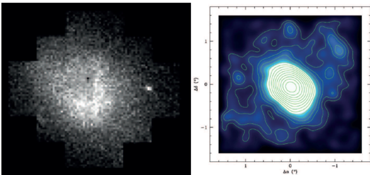
Fig. 7.— Structural irregularities in Fornax. Left: Grayscale map ( \sim 42' per side) of surface density of stars with 18.5 \leq V \leq 23 , from the photometry of Stetson et al. (1998, reproduced with permission from The University of Chicago Press). Notice the crescent-like feature near the center. Right: Smoothed stellar map from V, I photometry of Coleman et al. (2005b, reproduced by permission of the American Astronomical Society), who detect two shell-like features (one is visible \sim 1.3 deg northwest of the center) aligned with lobes along the morphological minor axis.
