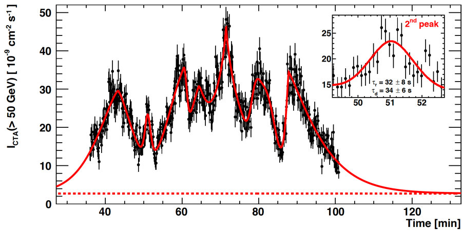
Figure 2. Simulated CTA light curve based on an extrapolation of the power spectrum for the strong 2006 VHE flare of the blazar PKS 2155-304. CTA will allow probing sub-minute timescales (see inlay) and thereby help to discriminate between different physical models. From [15].
