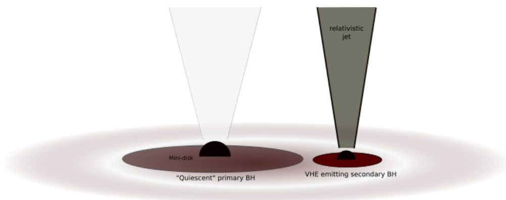
Figure 11. A possible binary black hole model for PKS 2155-304, with the binary (black holes plus mini-disks) being surrounded by a circumbinary disk. The tidal gas stream from this disk preferentially feeds the less massive, secondary black hole, whose jet emission dominates the observed VHE radiation spectrum. Both the short VHE variability and the high (apparent) luminosity can thus be accommodated, cf. [18].
