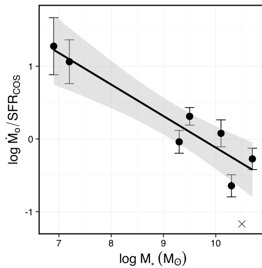
Figure 1. A fit to \eta \equiv \dot{M}/\text{SFR} vs. M_* for a sample of nearby GWs [36]. The gray region is the 95% confidence interval. Outflow masses have been estimated from multiple rest-frame UV absorption lines and photoionization modeling. Relationships between outflow and galaxy properties are key tools for connecting observations to theory. The fitted slope of -0.43 \pm 0.07 compares favorably with predictions from numerical simulations at low masses [38,39,41,42]. At higher masses the slope may be steeper, as suggested by some simulations [39,42] and measurements [23]. Reproduced with permission from Figure 1 of reference [36].
